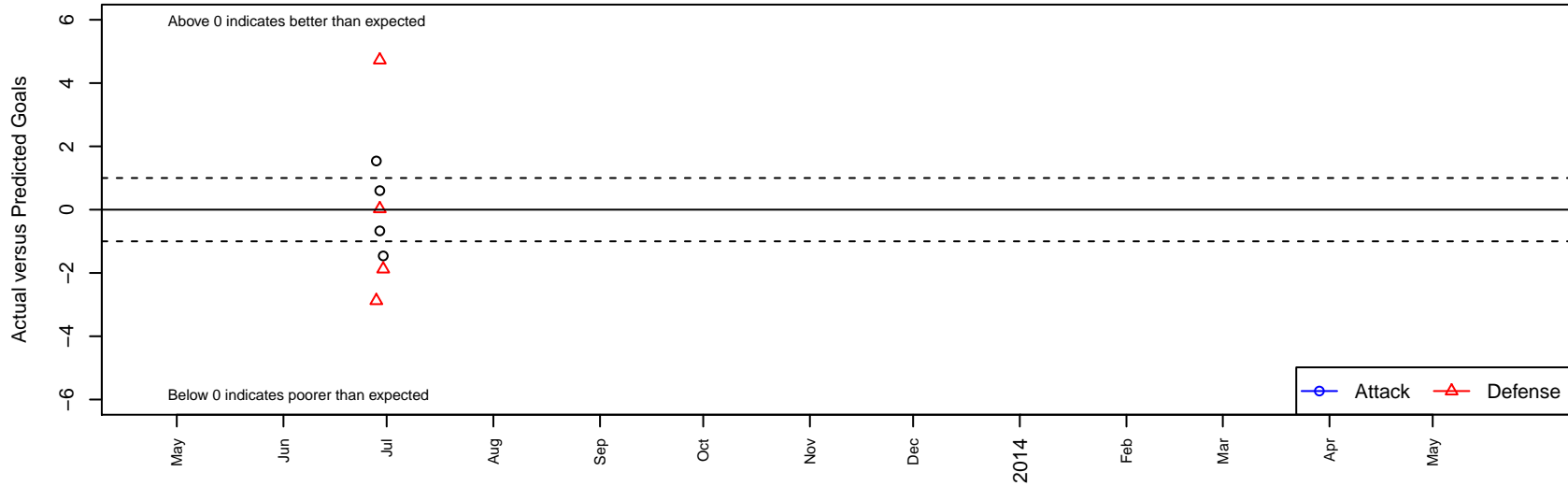
AYSO Lebanon United G02 Dots are actual minus expected GF (blue circles) and GA (red triangles). Blue line is smoothed change in attack strength. Red is smoothed change in defense strength.
